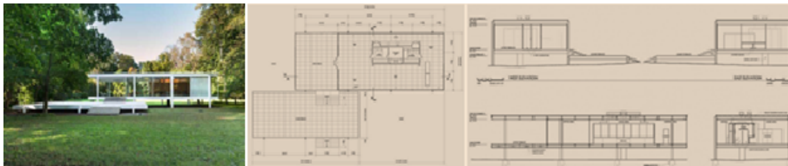
Görsel 4. Farnsworth House, Web kaynaklı görsel, plan ve kesitler (Archdaily, 2010)
