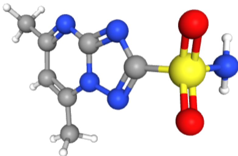
Figure 1. The optimized structure of title molecule.
